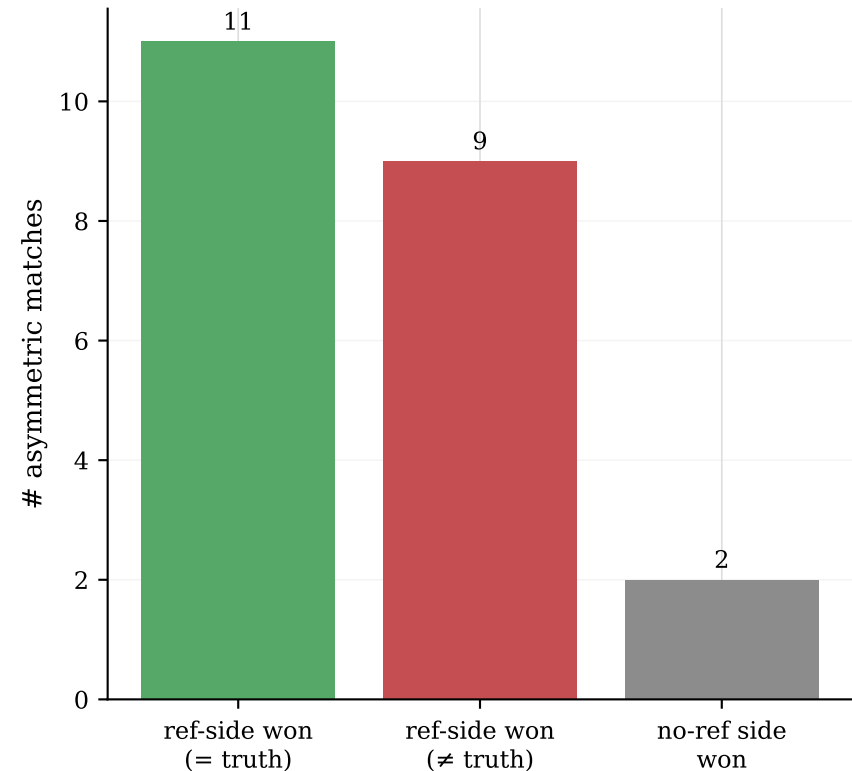
Outcome | asymmetric (n=22, ref-side wins 91%)
